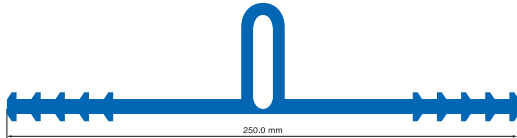
SPECTITE® PVC WS - IE 250 HD
